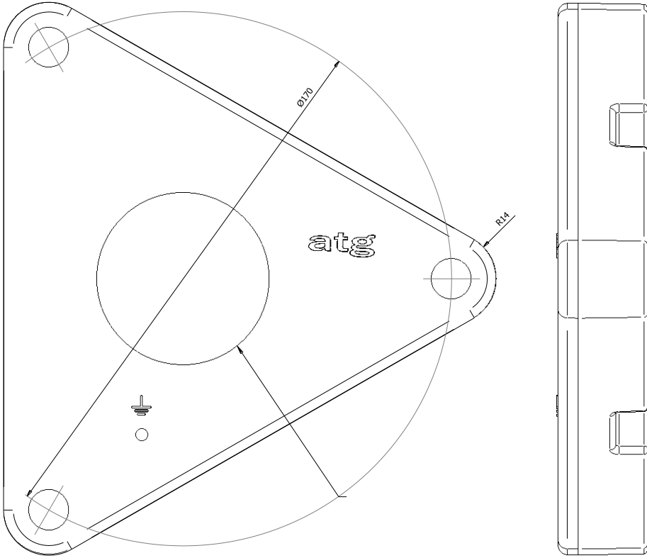
Figure 2.2 Mounting Foot
