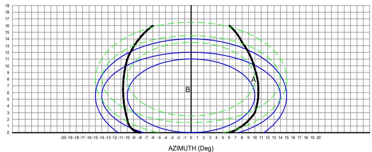
Intensity Chart - Runway Approach Luminaire - White
